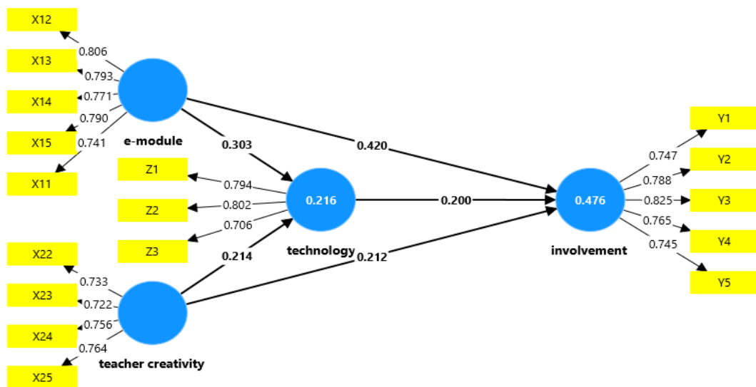
Figure 2. PLS-SEM results
