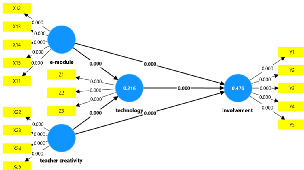
Figure 3. Bootstrapping results
