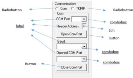
Figure 18. Serial connection module display
