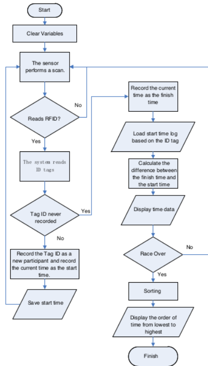
Figure 3. Planned system workflow
