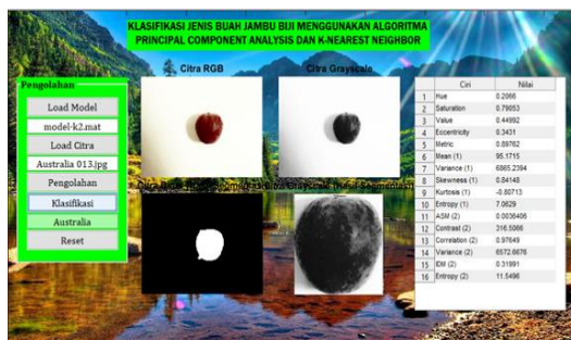
Gambar 6. Interface Program
