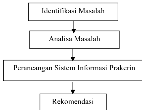
Gambar 1. Alur Penelitian
