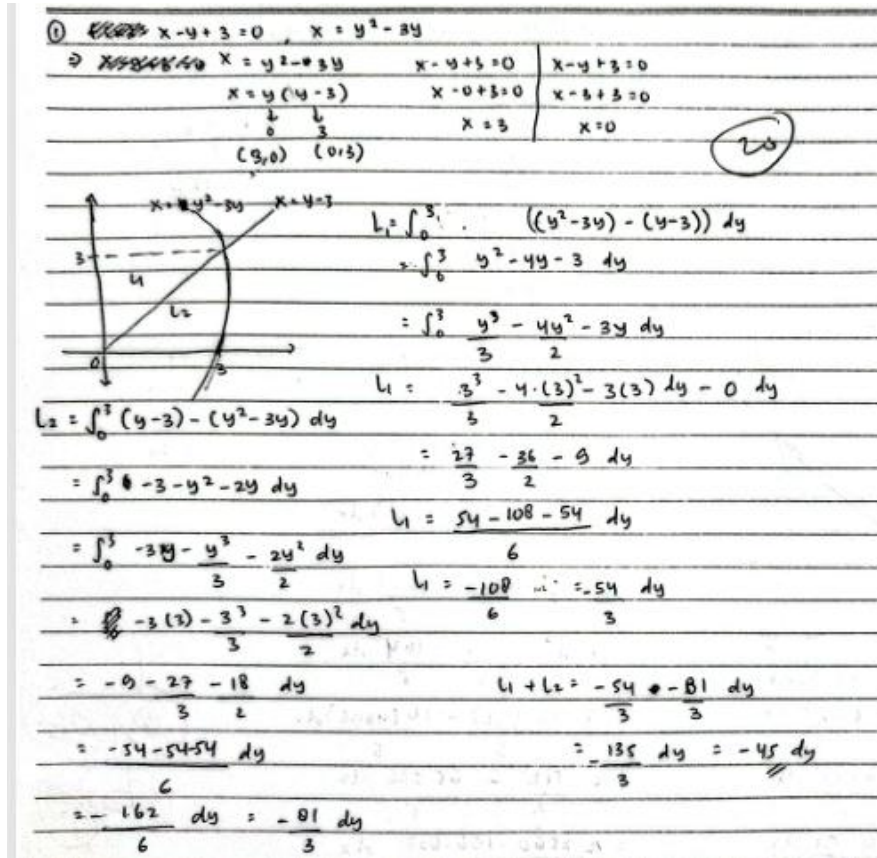
Gambar 1. Jawaban WMP
