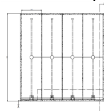
Gambar 6. Bak Sludge Drying Bed (SDB)
